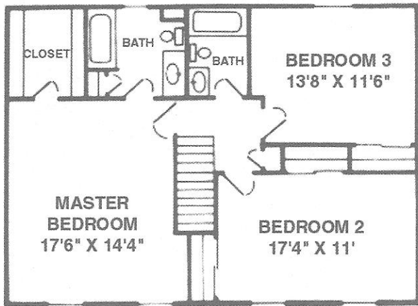
Standard second level floor plan
